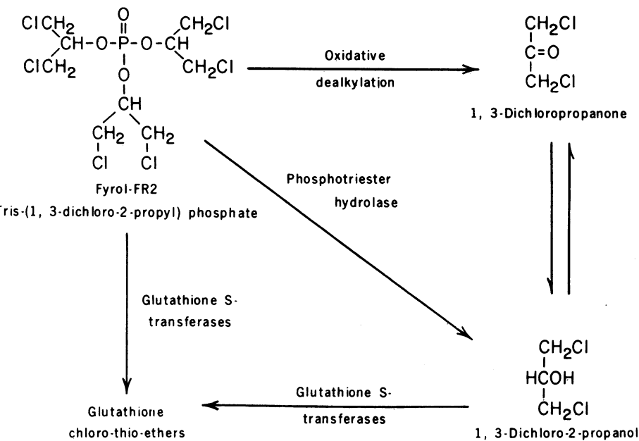
Fig. 2 (above right). Mutagenicity of Fyrol FR2, 1,3-dichloro-2-propanol, and 1,3-dichloro-2-propanone. All compounds were tested on Salmonella typhimurium strain TA100 as described (10). The number of spontaneous revertants (~150) has been subtracted from the revertant values plotted against the amount of mutagen. Where indicated, 20 \mu l of phenobarbital-induced mouse liver homogenate (fraction S-9) was incorporated into the pour plates. Fyrol FR2 was tested in six independent experiments with 20 \mu l of phenobarbital-induced mouse liver homogenate (fraction S-9). All showed positive dose response curves, and the mean and standard errors are indicated. The controls for the six experiments had a mean of 156 \pm 16 (standard error). The two different Fyrol FR2 samples (8) gave identical NMR spectra and mutagenicity results and have been averaged together. 1,3-Dichloro-2-propanol was less inhibitory to strain TA100 than Fyrol FR2; the mutagenicity kept increasing with dose (407 revertants per 250 \mu g; 937 revertants per 1000 \mu g). 1,3-Dichloro-2-propanol was also mutagenic in the presence of phenobarbital-induced rat liver homogenate, but not with PCB-induced rat liver homogenate. Fig. 3 (below right). Proposed metabolism of Fyrol FR2.
