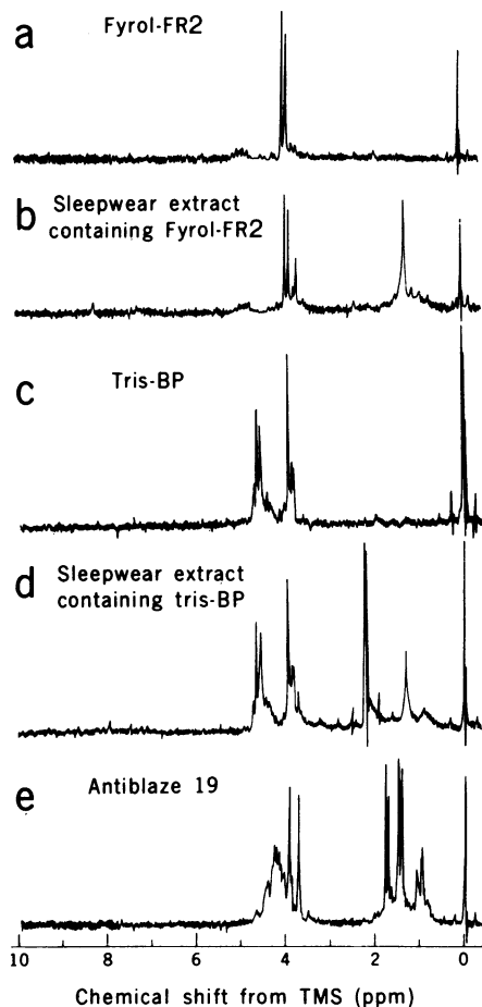
Fig. 1 (above left). Nuclear magnetic resonance spectra of (a) Fyrol FR2; (b) sleepwear extract containing Fyrol FR2; (c) tris-BP; and (d) extract of sleepwear containing tris-BP; (e) Antiblaze 19. A piece of each garment (100 cm 2 ) was extracted three times in 20 ml of acetone. If the fabric is a blend with acetate or triacetate it dissolves in the acetone. Therefore, to extracts of these fabrics we added an equal volume of hexane to precipitate the acetate. The precipitate was removed by filtration through Whatman No. 1 filter paper. The extracts were blown dry under nitrogen and the residues dissolved in 0.5 ml of deuterated chloroform with 1 percent tetramethylsilane (TMS) as a chemical shift marker. The NMR spectra were obtained on a Varian T60 spectrometer.
